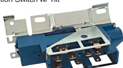
GF1086 NEW 1969-83 Ignition Switch w/ Tilt
